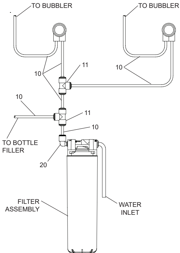
Figure 3 - LZLMSN-EDFPVM217DK Tube Routing
