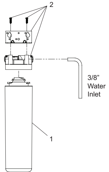
Filter Head Assembly used after 01/01/2021
