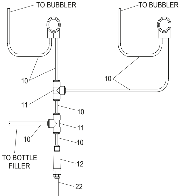
Figure 2 - EZLMSN-EDFPVM217DK Tube Routing
