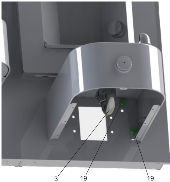
Figure 4 - Upper Panel Installation
