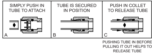
Figure 11 – Quick Connect Fittings
