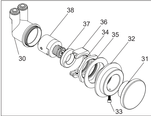
Figure 10 - Bottle Filler Push Button Assembly
