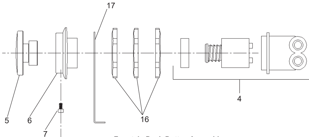
Fountain Push Button Assembly
