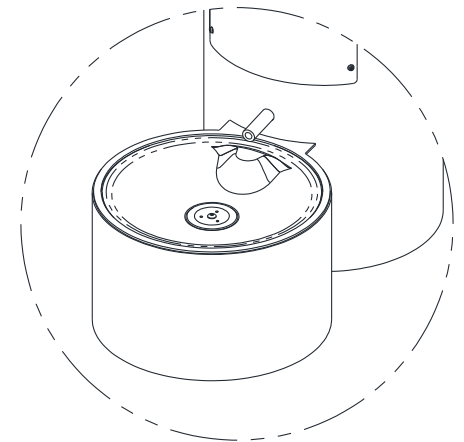
OPTIONAL -PF PET FOUNTAIN DETAIL
